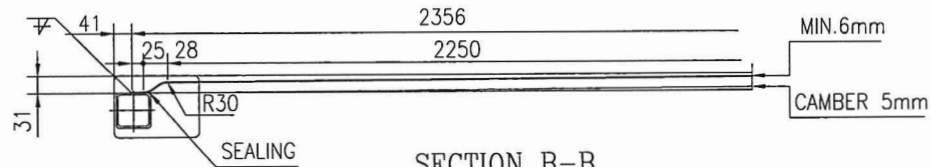
SECTION B-B 1:10
