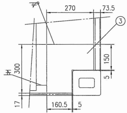
DETAIL F 1:10
