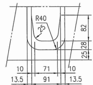
DETAIL D 1:5
