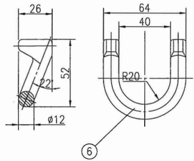
DETAIL OF LASHING RING 1:2
