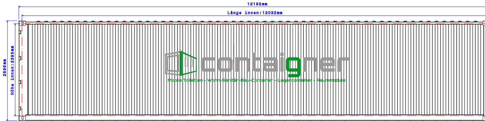
Front view
