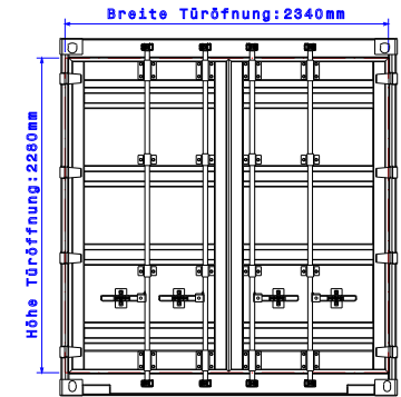
Left view
